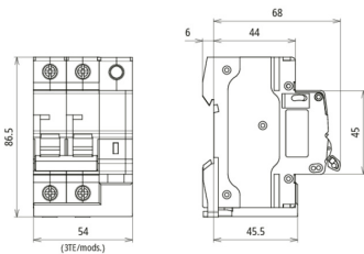
Dimension drawing MCB+POP 16A 1P+N
