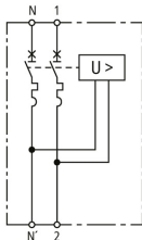
Basic circuit diagram MCB+POP 16A 1P+N
