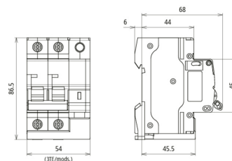
Dimension drawing MCB+POP 25A 1P+N
