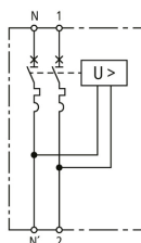
Basic circuit diagram MCB+POP 32A 1P+N
