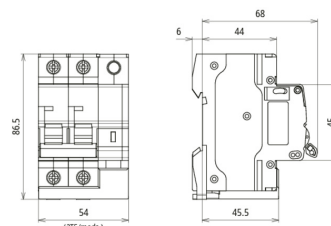
Dimension drawing MCB+POP 50A 1P+N
