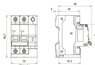
Dimension drawing MCB+POP 63A 1P+N
