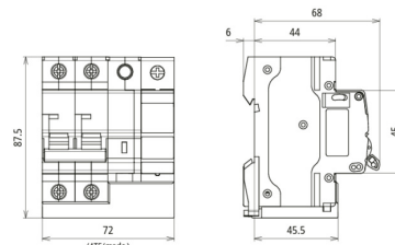
Dimension drawing MCB+POP+SPD 16A 1P+N
