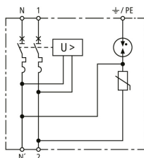
Basic circuit diagram MCB+POP+SPD 25A 1P+N
