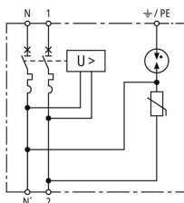
Basic circuit diagram MCB+POP+SPD 32A 1P+N
