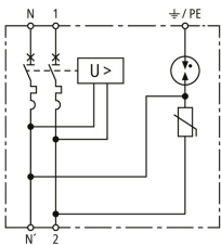
Basic circuit diagram MCB+POP+SPD 40A 1P+N
