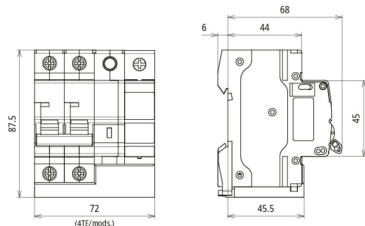
Dimension drawing MCB+POP+SPD 40A 1P+N
