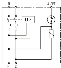
Basic circuit diagram MCB+POP+SPD 50A 1P+N
