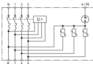
Basic circuit diagram MCB+POP+SPD 16A 3P+N
