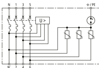
Basic circuit diagram MCB+POP+SPD 20A 3P+N
