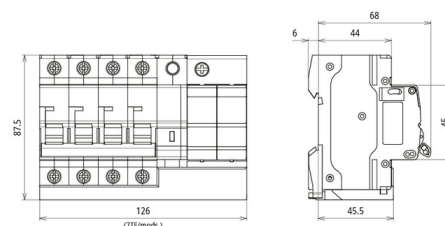
Dimension drawing MCB+POP+SPD 20A 3P+N
