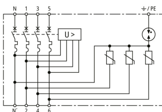
Basic circuit diagram MCB+POP+SPD 32A 3P+N
