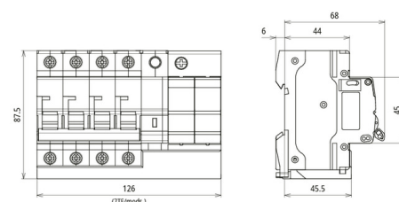
Dimension drawing MCB+POP+SPD 32A 3P+N
