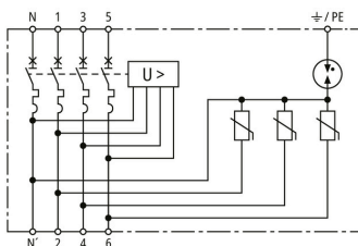
Basic circuit diagram MCB+POP+SPD 63A 3P+N
