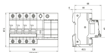
Dimension drawing MCB+POP+SPD 63A 3P+N
