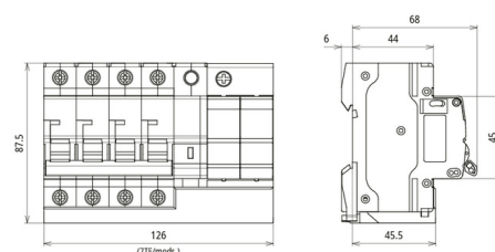
Dimension drawing MCB+POP+SPD 80A 3P+N
