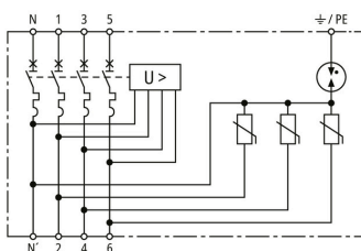
Basic circuit diagram MCB+POP+SPD 80A 3P+N
