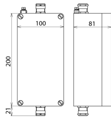
Dimensions ALGA 5
