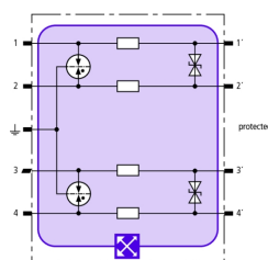
Basic circuit diagram BXT ML4 BD 5
