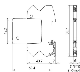
Dimension drawing BCO ML2 BD HC5A 24
