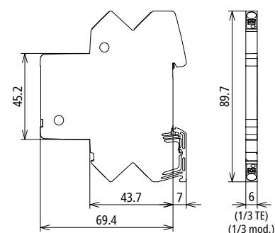
Dimension drawing
