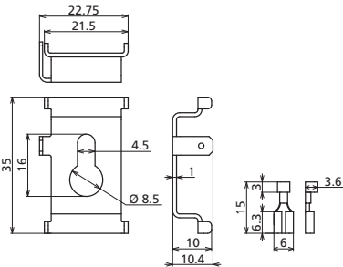
Dimension drawing
