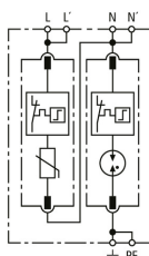
Basic circuit diagram DG MP TT 2P 275
