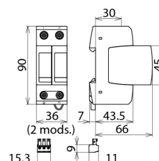
Dimension drawing DG MP TT 2P 275
