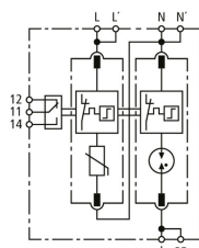
Basic circuit diagram DG MP TT 2P 275 FM
