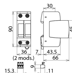
Dimension drawing DG MP TT 2P 275 FM
