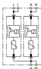
Basic circuit diagram DG MP TN 275
