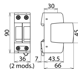
Dimension drawing DG MP TN 275
