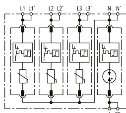
Basic circuit diagram DG MD TT 275
