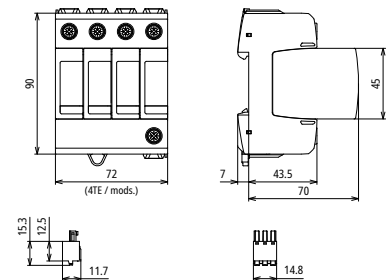
Dimension drawing
