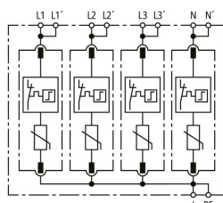
Basic circuit diagram DG MD TNS 275
