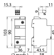
Dimensions DG 1000 FM
