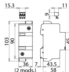
Dimension drawing DG 1000 FM
