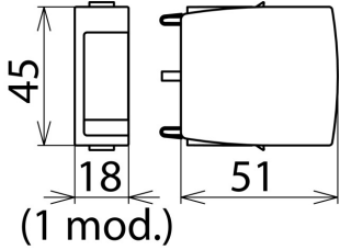
Dimensions DG MOD PV SCI 75
