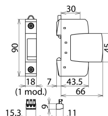
Dimensions DG S WE 600
