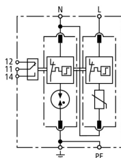
Basic circuit diagram DG M TT 2P 275 NL FM
