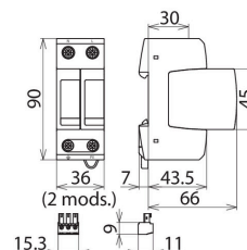
Dimension drawing DG M TT 2P 275 NL FM
