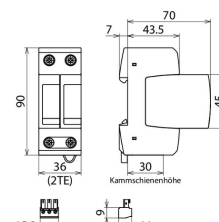
Dimension drawing DG M TT 2P ACI 385 FM
