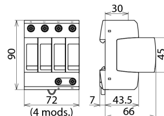
Dimension drawing DG M TT 275 NL
