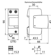
Dimension drawing DV M2 TT 2P 255 FM
