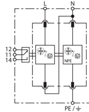
Basic circuit diagram DV M2 TT 2P 255 FM
