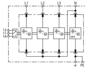
Basic circuit diagram DV M2 TT 255 FM
