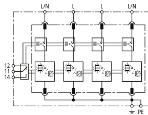
Basic circuit diagram DV ACI M TNS 264 FM
