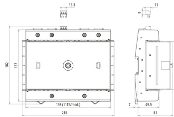
Dimension drawing DV ACI M TNS 264 FM
