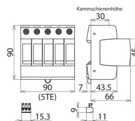
Dimensions DG M PV2 SCI SN1868
